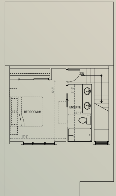
UPPER LEVEL 358 SQ.FT
