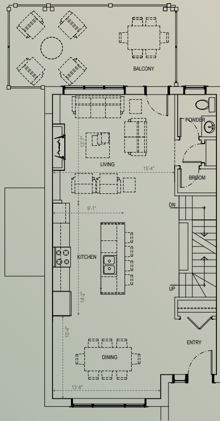
MAIN LEVEL 862 SQ.FT
