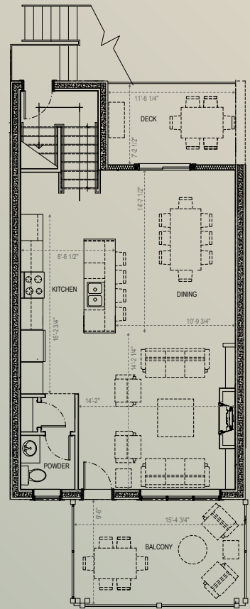
LIVING LEVEL 664.76 SQ.FT.
